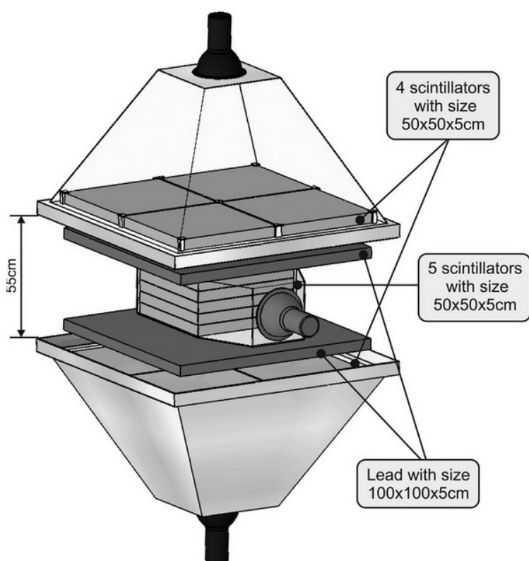
Figure 2 Basic detecting unit of the SEVAN network.
