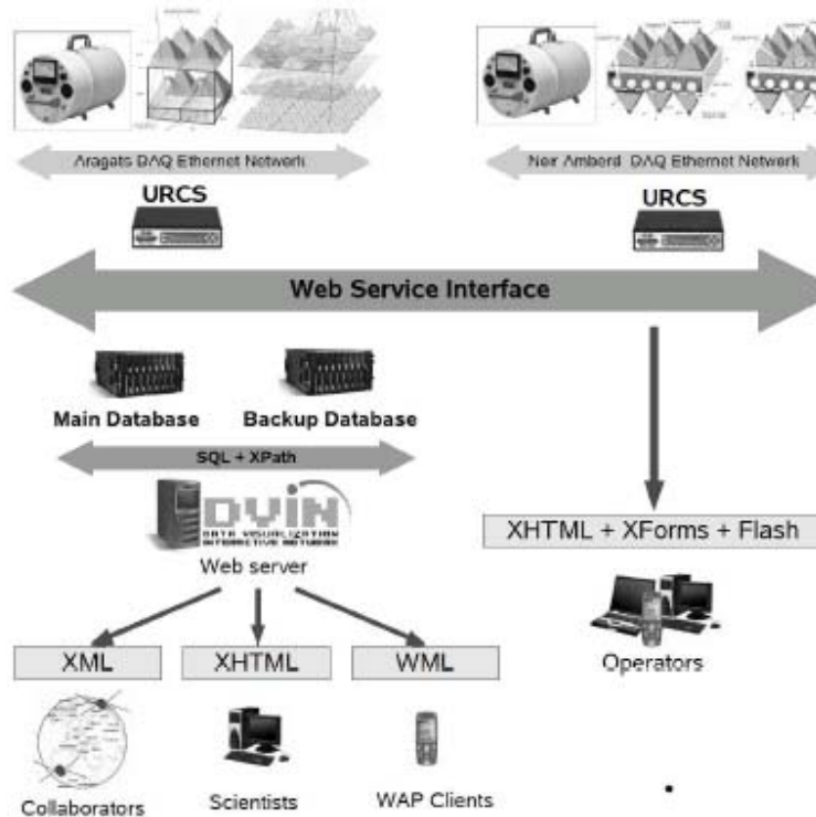
Figure 4 Layout of the new ASEC data acquisition system. Several detector arrays are operating at Nor-Amberd and Aragats research stations. The detectors are controlled by URCS which are installed on each station. The data dissemination and detector control is performed by web services. The DVIN is used to distribute the data to end users.
