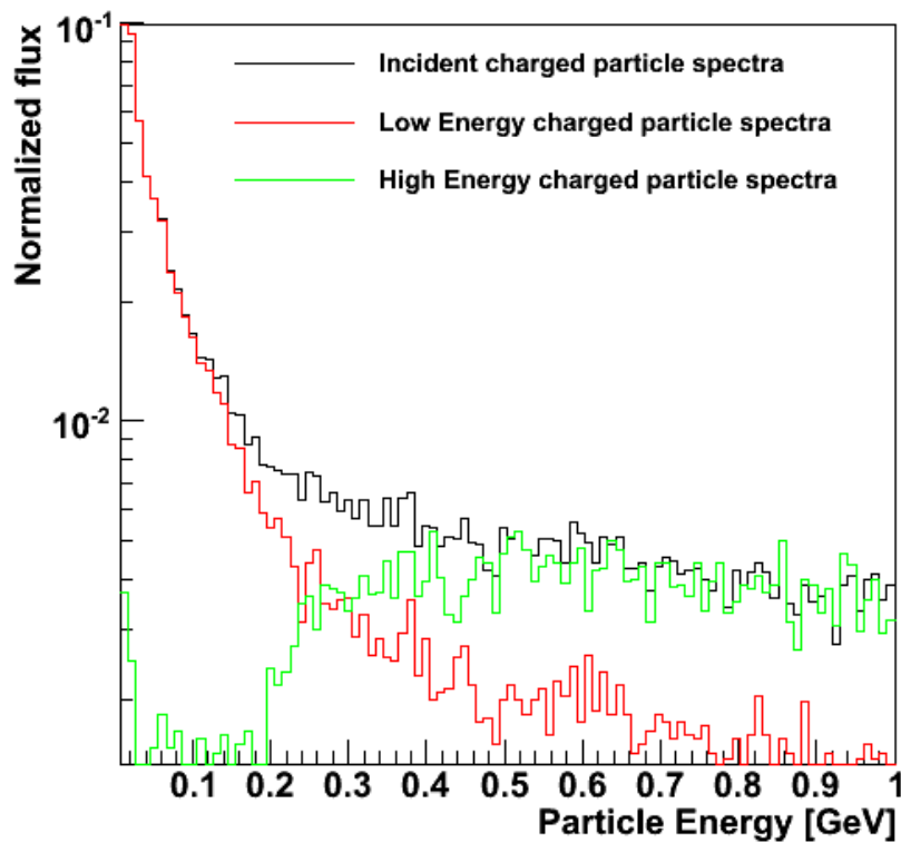
Figure 5 Energy spectra of low and high energy charged particles as measured by first and third layer of SEVAN module (simulation)
